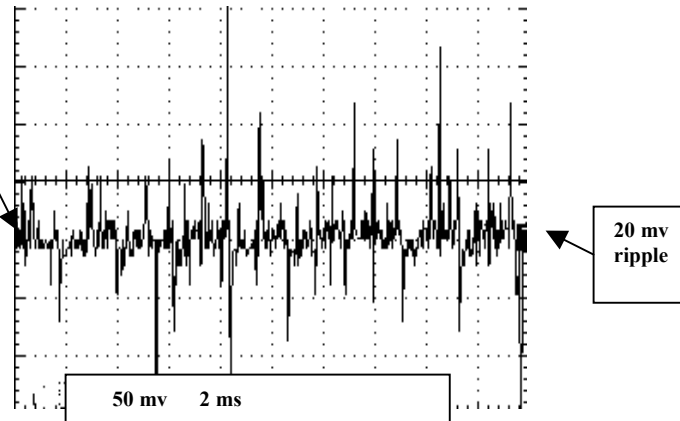
Ripple on 2 V cell
